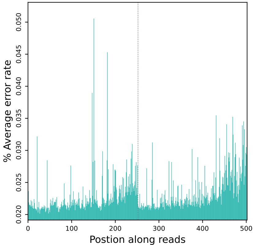
Error rate distribution along reads (R10903)
